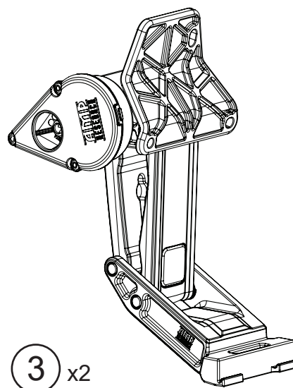
Motor linkage assembly
