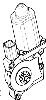
10 x2 Motor
