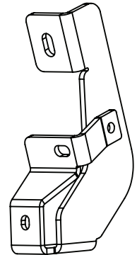
25 x2 Rail Mounting Bracket
