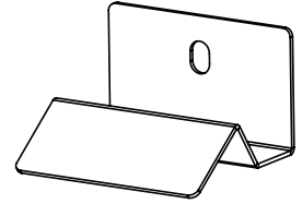
17 x4 LED Light Bracket
