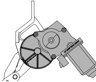
Drive Linkage (Front) Motor Angle
