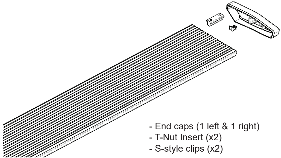
① x2 Running Board assembly
