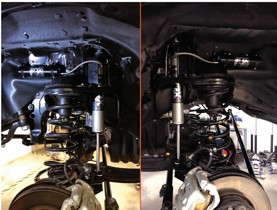
Figure 7: Left and right front Performance Remote Reservoir shocks installed
