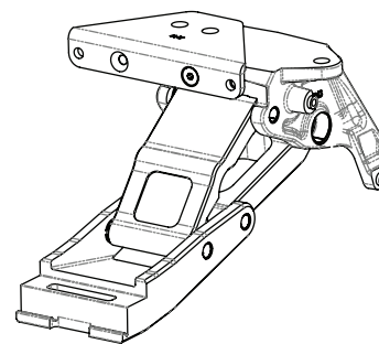
3b Rear Idler Linkage
