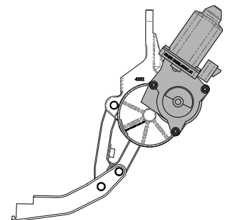
Passenger's Motor Install Orientation
