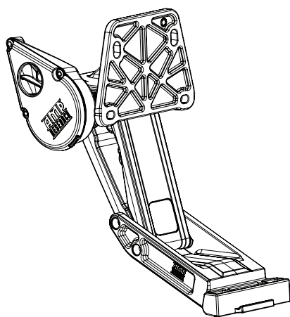
2 Motor Linkage assembly Driver
